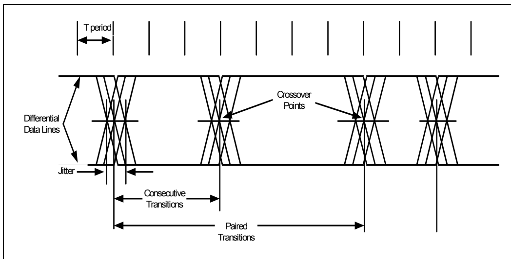
Figure 33-29. USB Jitter
