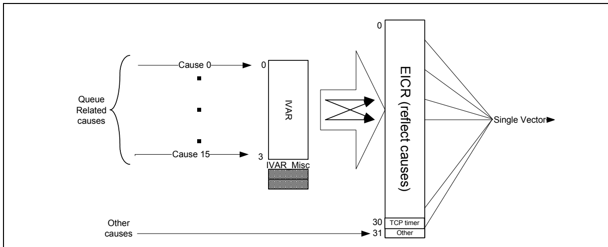
Figure 26-20. Cause Mapping in Legacy Mode
