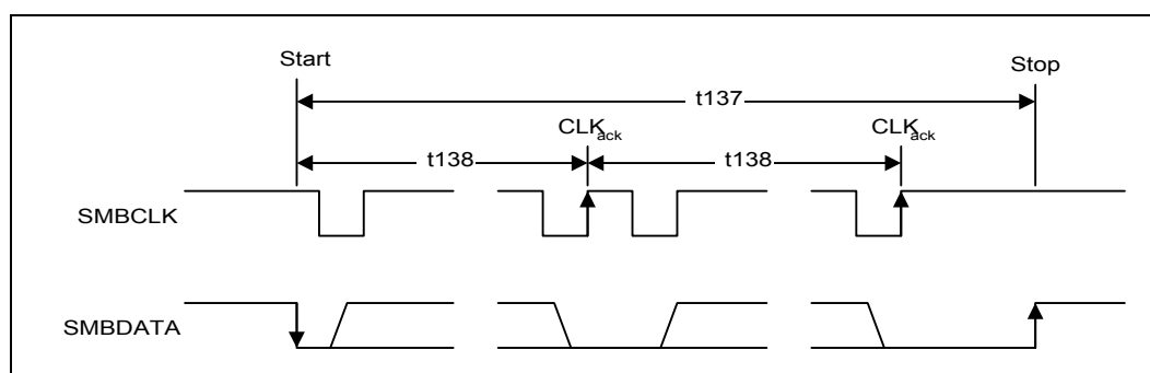
Figure 33-32.SMBus Timeout
