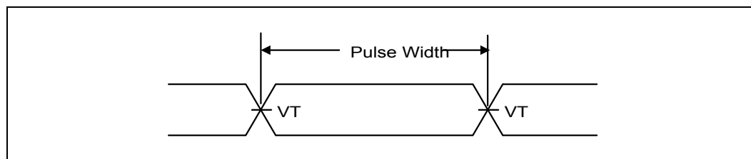
Figure 33-26. Pulse Width
