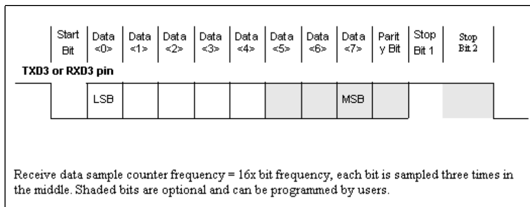
Figure 4-17. Example UART Data Frame
