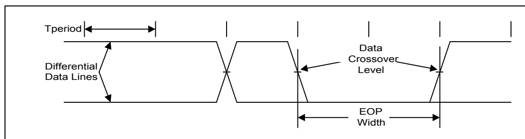
Figure 33-31.SMBus Transaction
