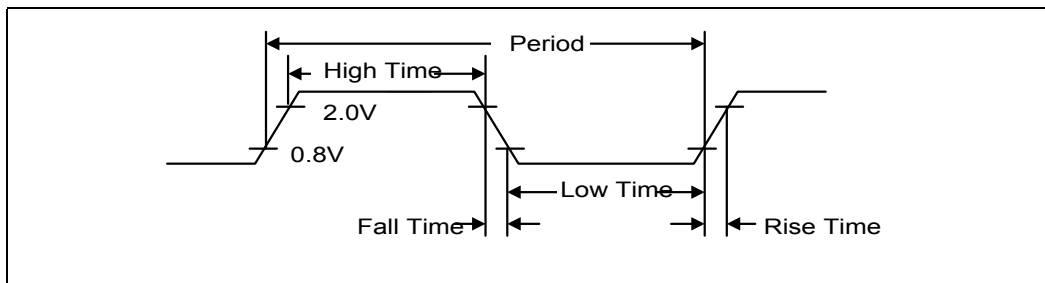
Figure 33-22. Clock Timing
