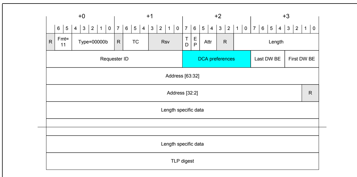
Figure 26-27. PCIe Message Format for DCA
