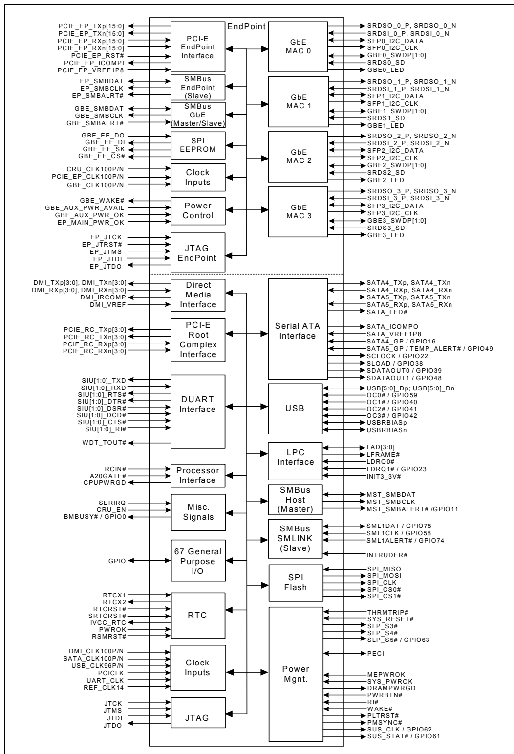
Figure 32-1. Interface Signals Block Diagram
