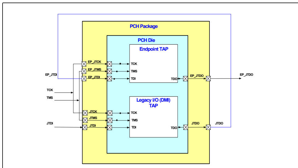
Figure 30-1. TAP Connectivity
