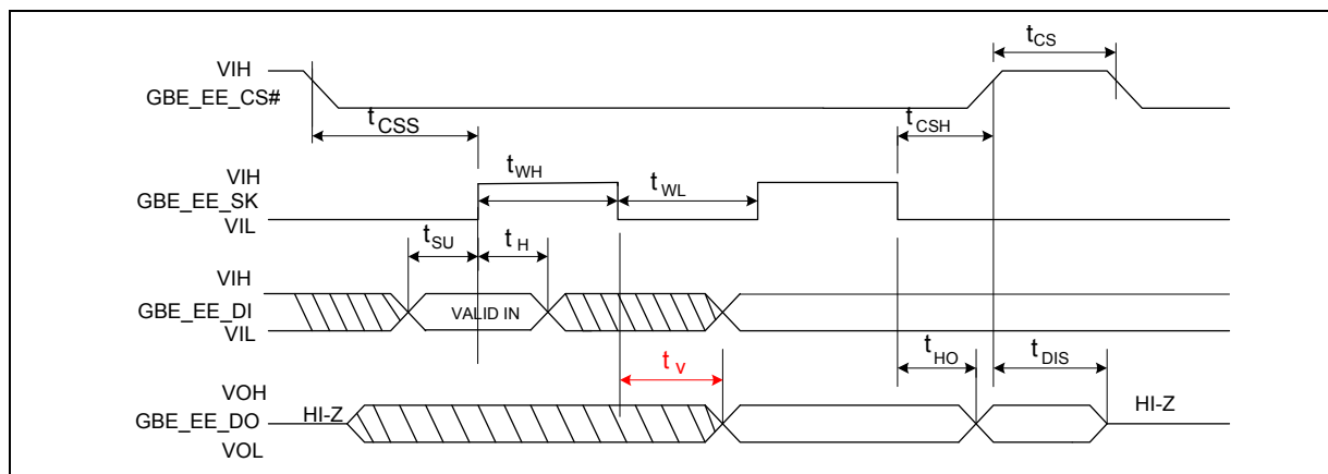
Figure 33-19.EEPROM Timing Diagram
