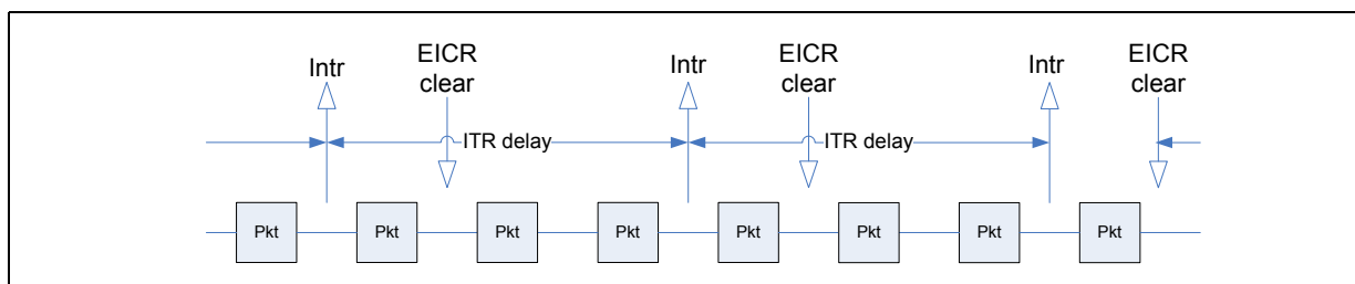
Figure 26-23. Case A: Heavy Load, Interrupts Moderated
