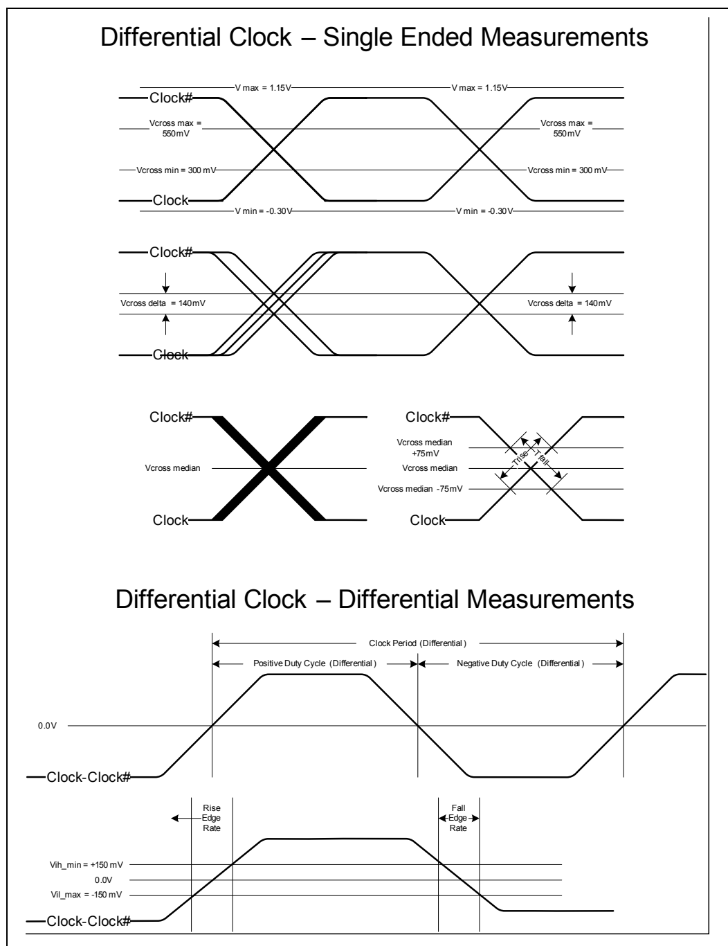
Figure 33-34. Measurement Points for Differential Waveforms
