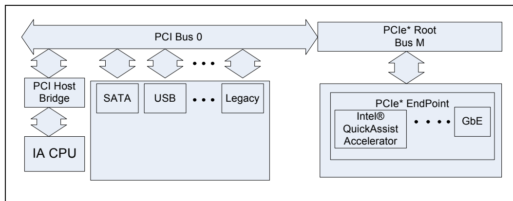
Figure 3-1. Device-Centric Logical View of PCH Devices
