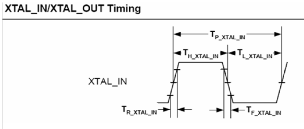
Figure 7. XTAL Timing Diagram
