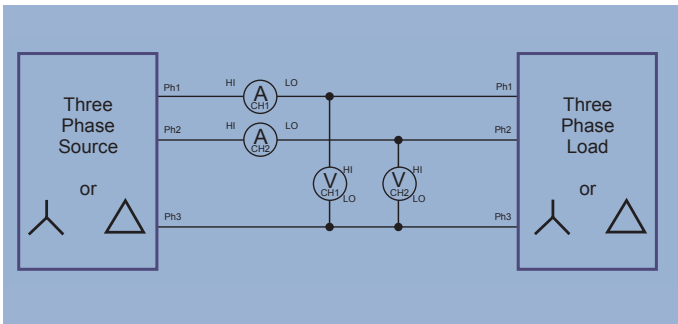
Figure 13. Three-phase, three-wire, 2 wattmeter method.
