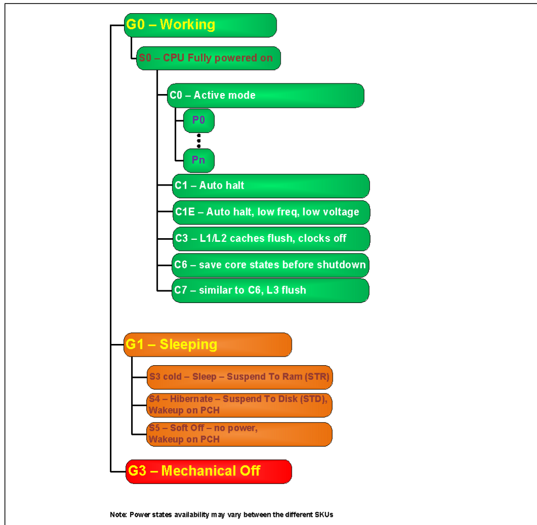
Figure 4-1. Processor Power States
