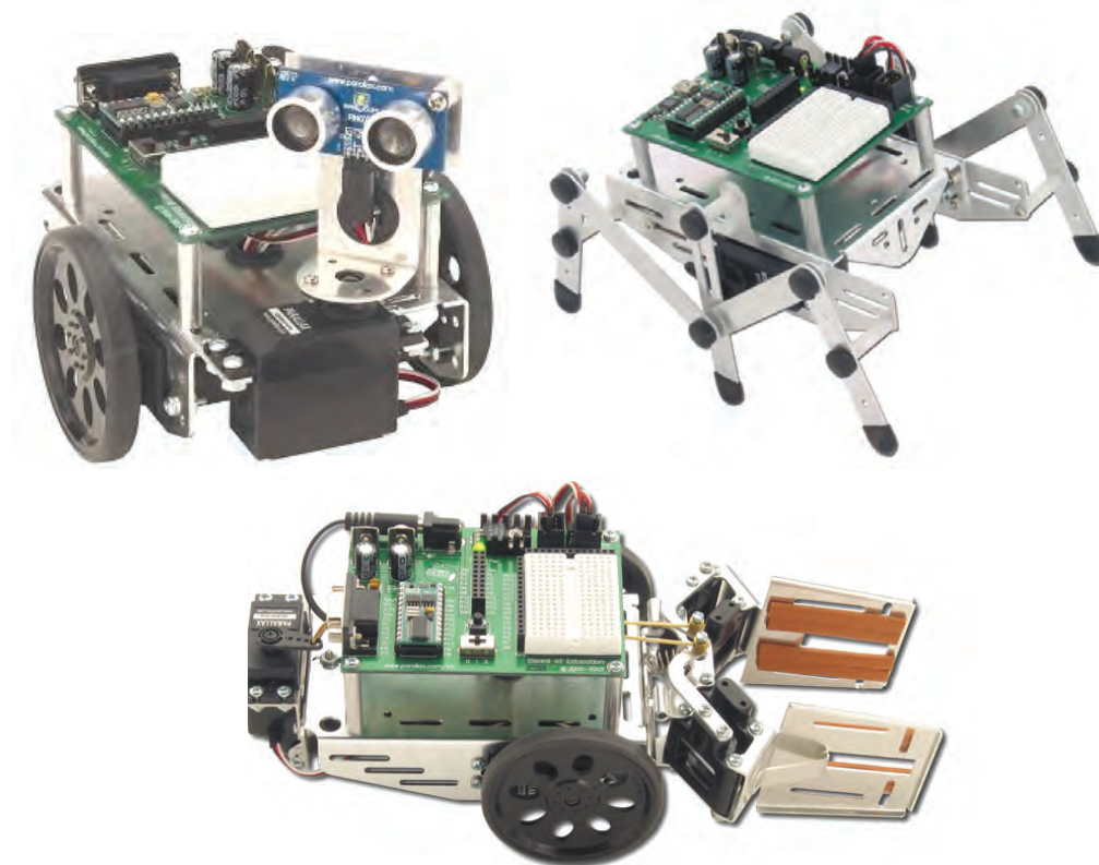
Figure 8-14: Ping))) Sensor and Bracket, Crawler Legs, and Gripper Add-Ons
