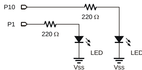
Figure 5-9 LED Whisker Testing Schematic
