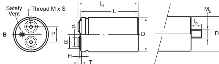
Fig. 2 B: High current M6 disc: Screw terminal (ST) and screw terminal bolt nut (STB)
