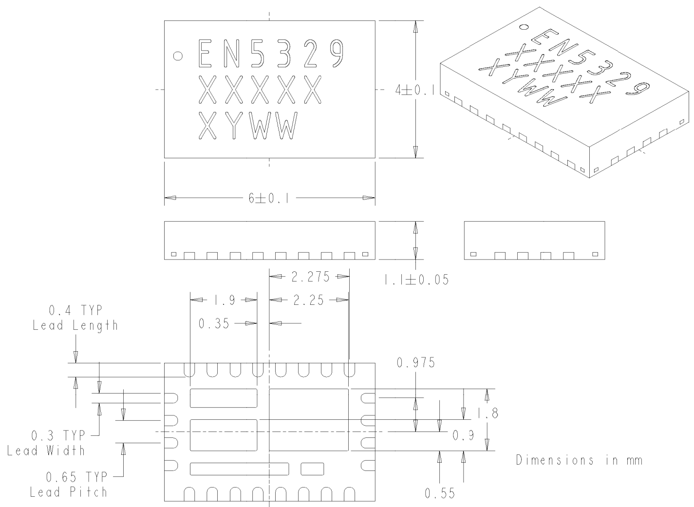
Figure 11. EN5329QI Package Dimensions (Bottom View)
