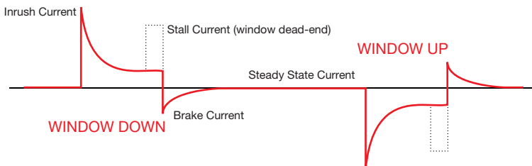
LOAD CURRENT (One Motor)
