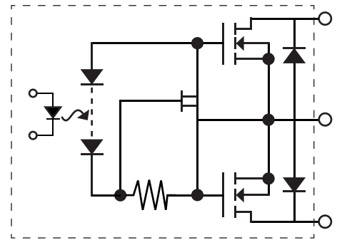
PhotoMOS Internal Construction
