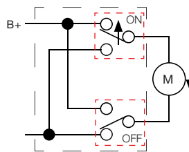
Contact 1 Turns On
