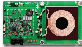
bq500211A eval board with 12V coil.
