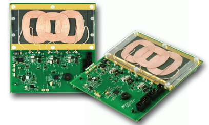
bq500410A eval board with 12V coil array.
