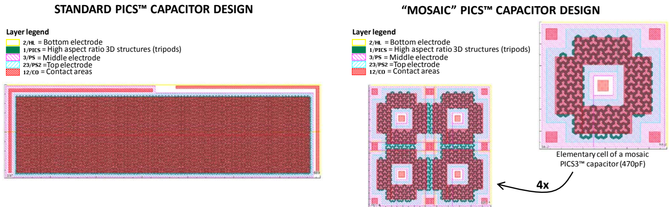
Figure 5: Standard PICS capacitor design compared with Mosaic PICS capacitor design. The ESR is driven by the capacitor shape/outer extend in the standard design when it depends on the localized element in the Mosaic. ESR_{Global} becomes a variation of 1/N in the second case, N being the number of elementary cells parallelized.
