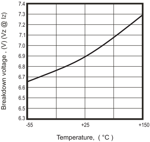
Fig. 1 - Typical breakdown votage versus temperature
