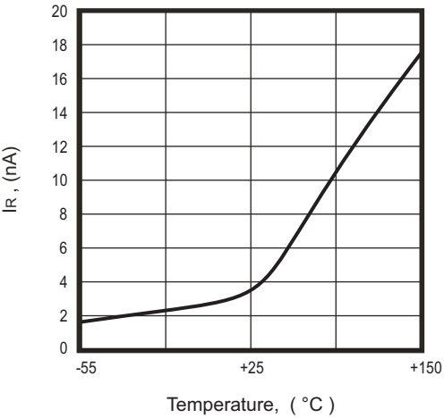
Fig. 2 - Typical leakage current versus temperature
