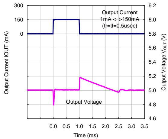
VR=5.0V, C_{OUT}=10\mu\text{F}
