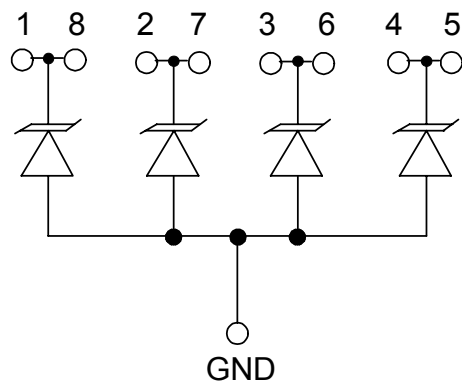
Device Schematic
