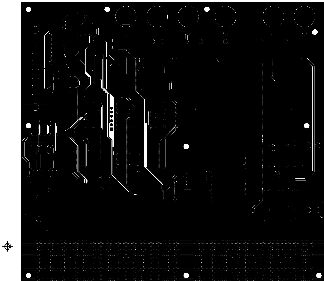
Figure 13. Bottom Side
