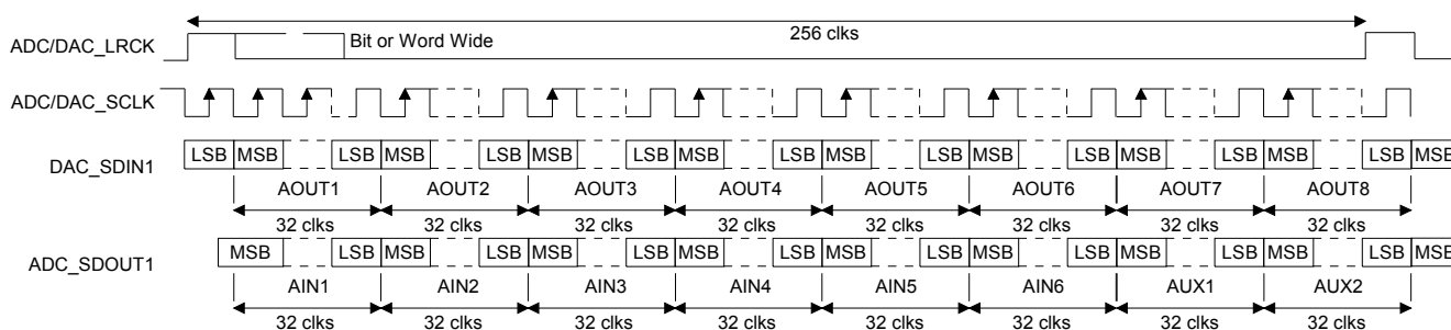
Figure 20. TDM Format
