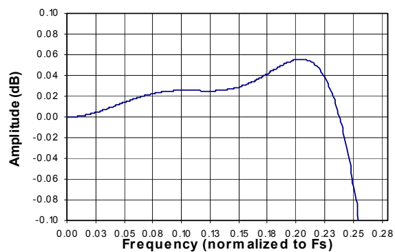
Figure 43. QSM Passband Ripple
