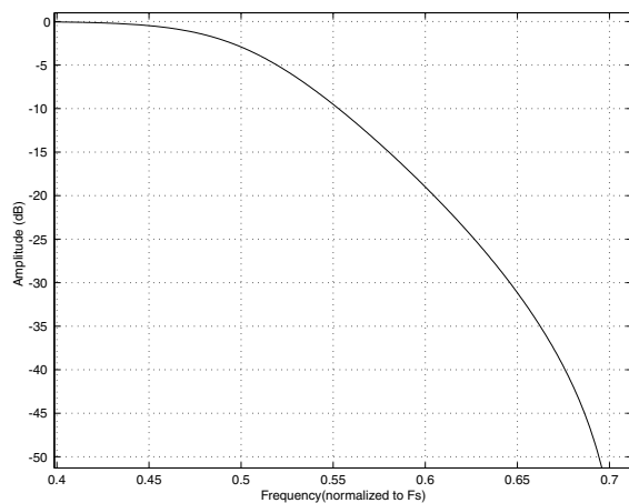
Figure 54. QSM Transition Band (detail)
