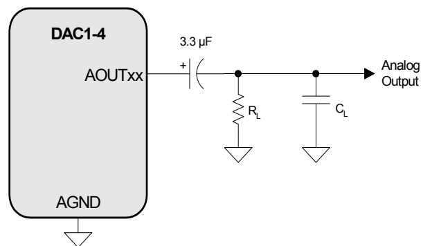
Figure 2. Output Test Circuit for Maximum Load
