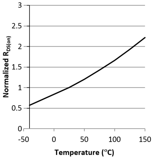
GS61008P R_{DS(on)} Temperature Dependence
