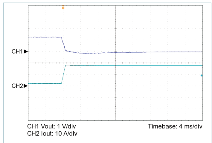
Figure 8 — 10% to 100% load transient response, V_{IN} = 300\text{ V} , nominal trim, C_{OUT\_EXT} = 200\text{ }\mu\text{F}
