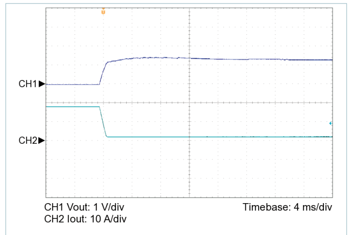
Figure 7 — 100% to 10% load transient response, V_{IN} = 300\text{ V} , nominal trim, C_{OUT\_EXT} = 200\text{ }\mu\text{F}
