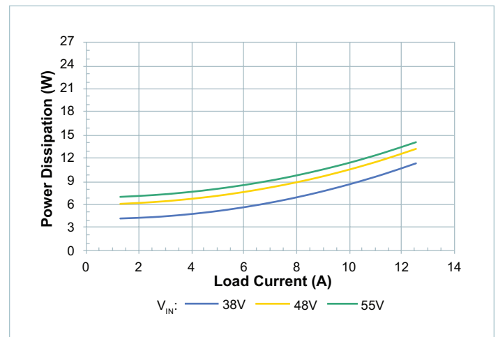
Figure 7 — Power dissipation at T_{CASE} = 25^{\circ}\text{C}
