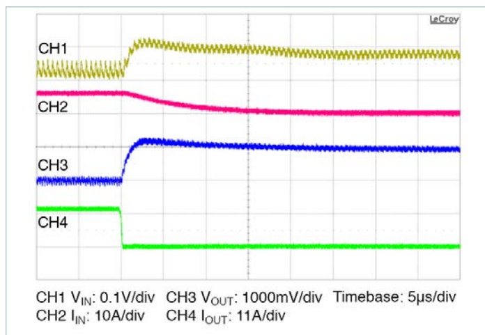
Figure 15 — 12.5 – 0A transient response: C_{IN} = 330\mu\text{F} , I_{IN} measured prior to C_{IN} , no external C_{OUT}
