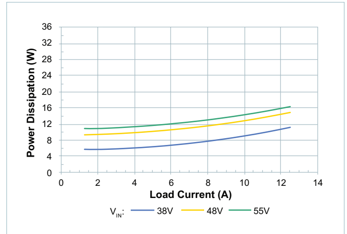
Figure 5 — Power dissipation at T_{CASE} = -40^{\circ}\text{C}
