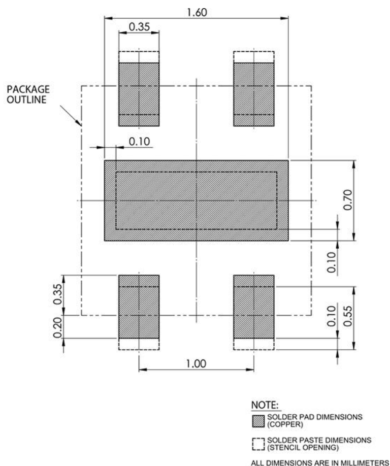
Figure 9 Recommended metal land pattern for STSC1 (all dimensions are in mm). Recommended solder paste stencil thickness is 100µm, pads on PCB are recommended to be non solder mask defined (NSMD).
