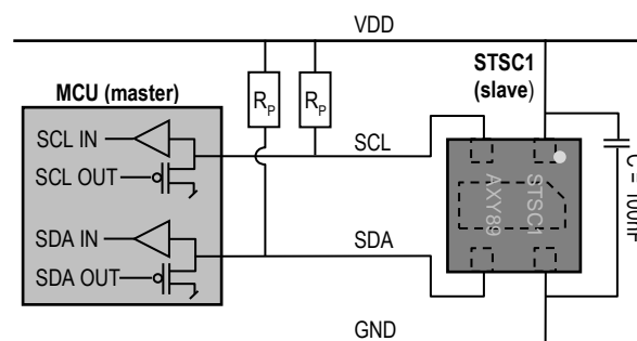
Figure 4 Typical application circuit, including pull-up resistors R_P and decoupling of VDD and VSS by a capacitor.
