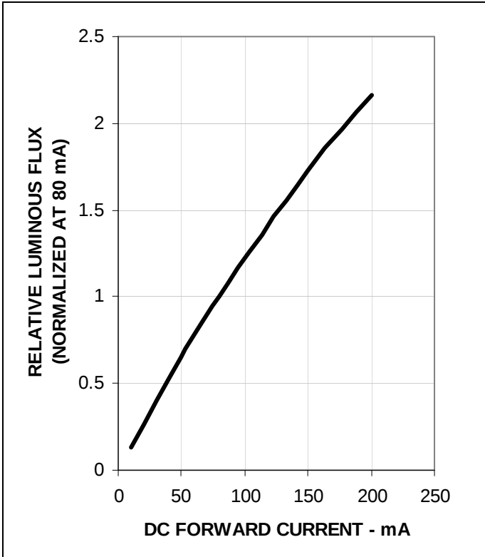
Relative Luminous Flux vs. Forward Current
