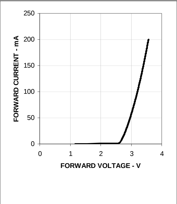
Forward Current vs. Forward Voltage
