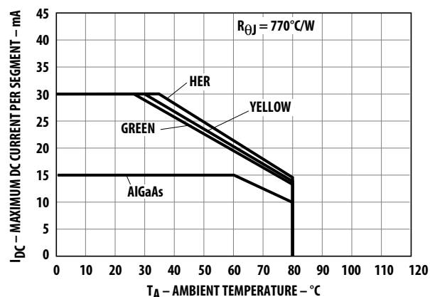
Figure 4. Maximum allowable DC current vs. ambient temperature.
