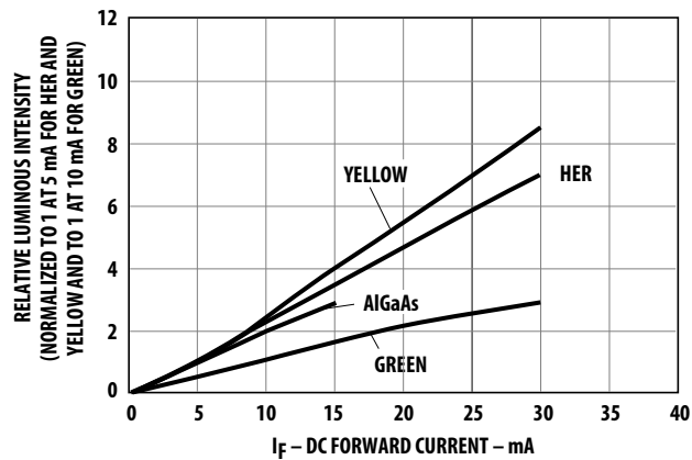
Figure 6. Relative luminous intensity vs. DC forward current.
