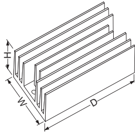
Vertical type
