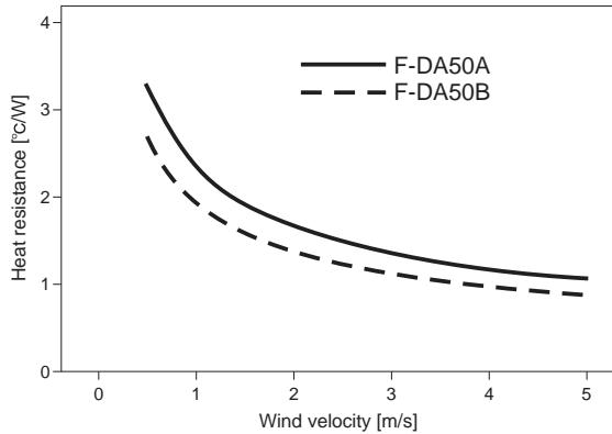
Fig.1 F-DA50A, F-DA50B Heat sink heat resistance
