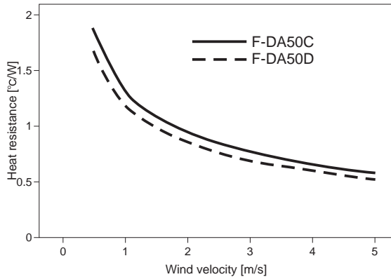
Fig.2 F-DA50C, F-DA50D Heat sink heat resistance
