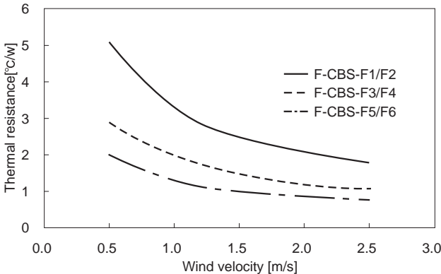
Fig.7 Thermal resistance of heat sink(Forced air)
