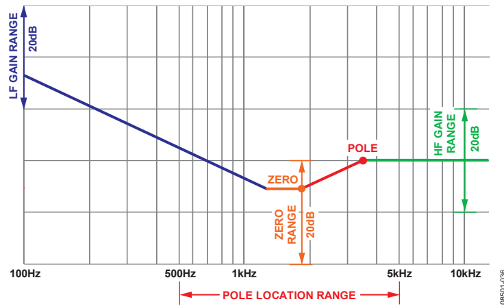
Figure 37. Digital Filter Programmability
