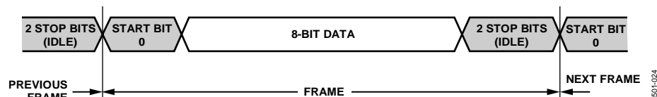
Figure 24. Digital Current Share Frame Timing Diagram
