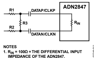
Figure 11. Attenuation Circuit
