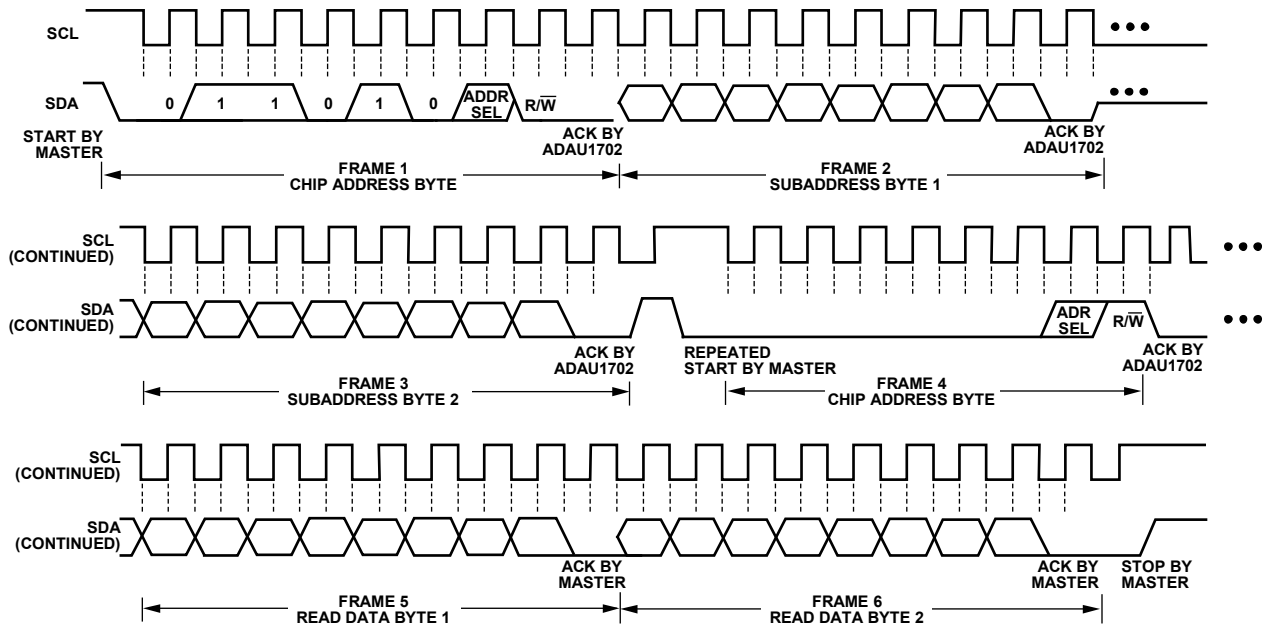
Figure 21. I 2 C Read from ADAU1702 Clocking
