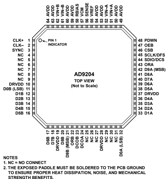
Figure 5. Pin Configuration
