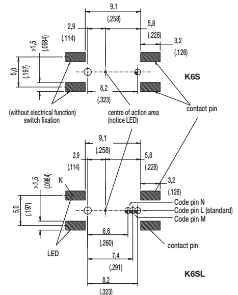
PCB LAYOUT, MOUNTING SIDE
