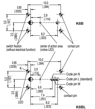
PCB LAYOUT, MOUNTING SIDE
