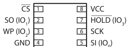
Figure 1-2. 8-UDFN (Top View)
