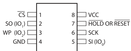
Figure 1-1. 8-SOIC (Top View)
