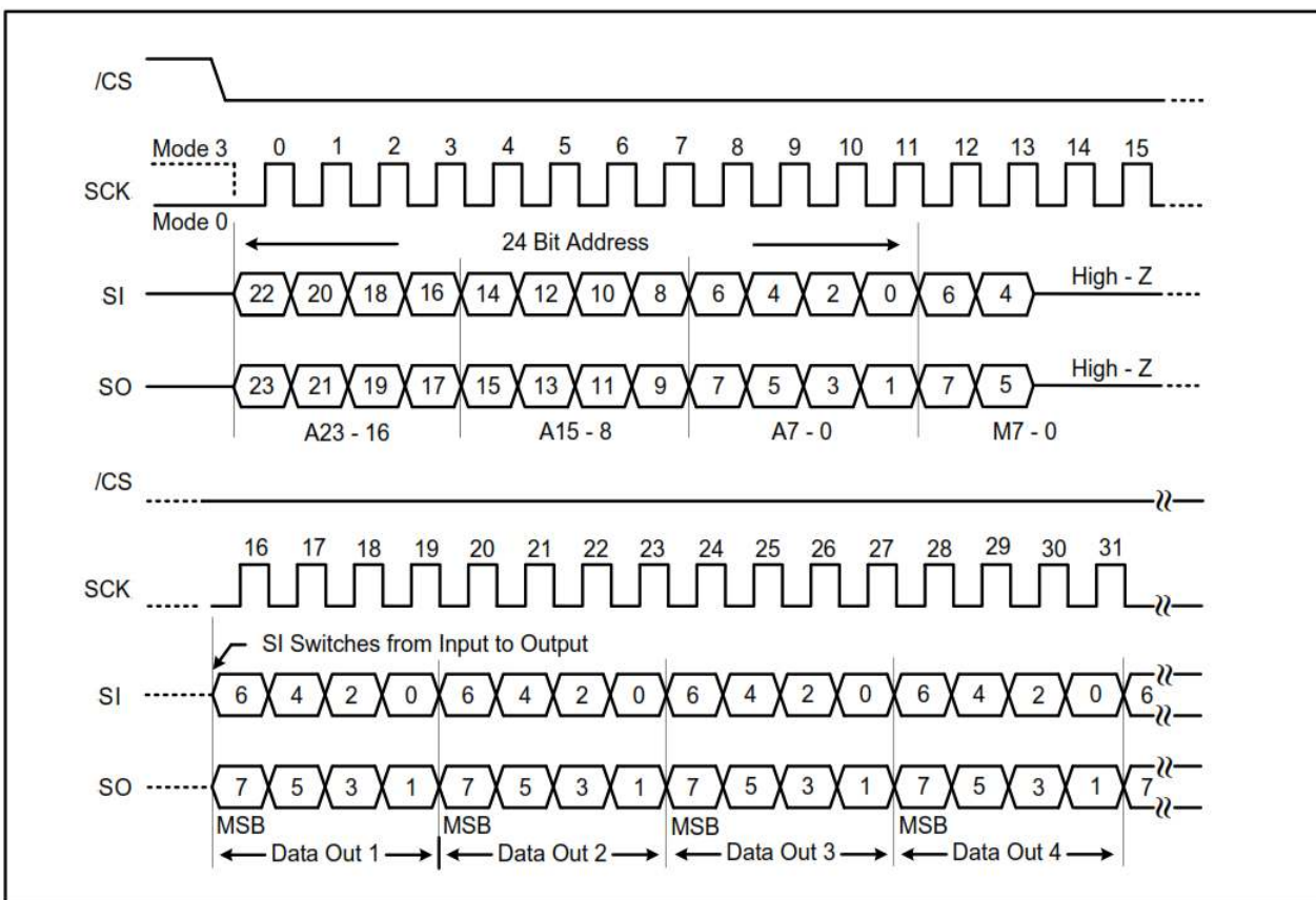
Figure 7-17. Fast Read Dual I/O Instruction (previous M7-0 = Axx)
