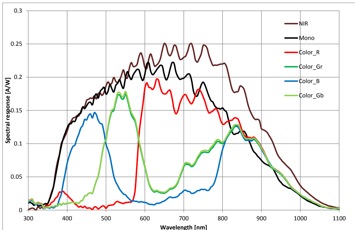
FIGURE 65: TYPICAL SR VS. WAVELENGTH
