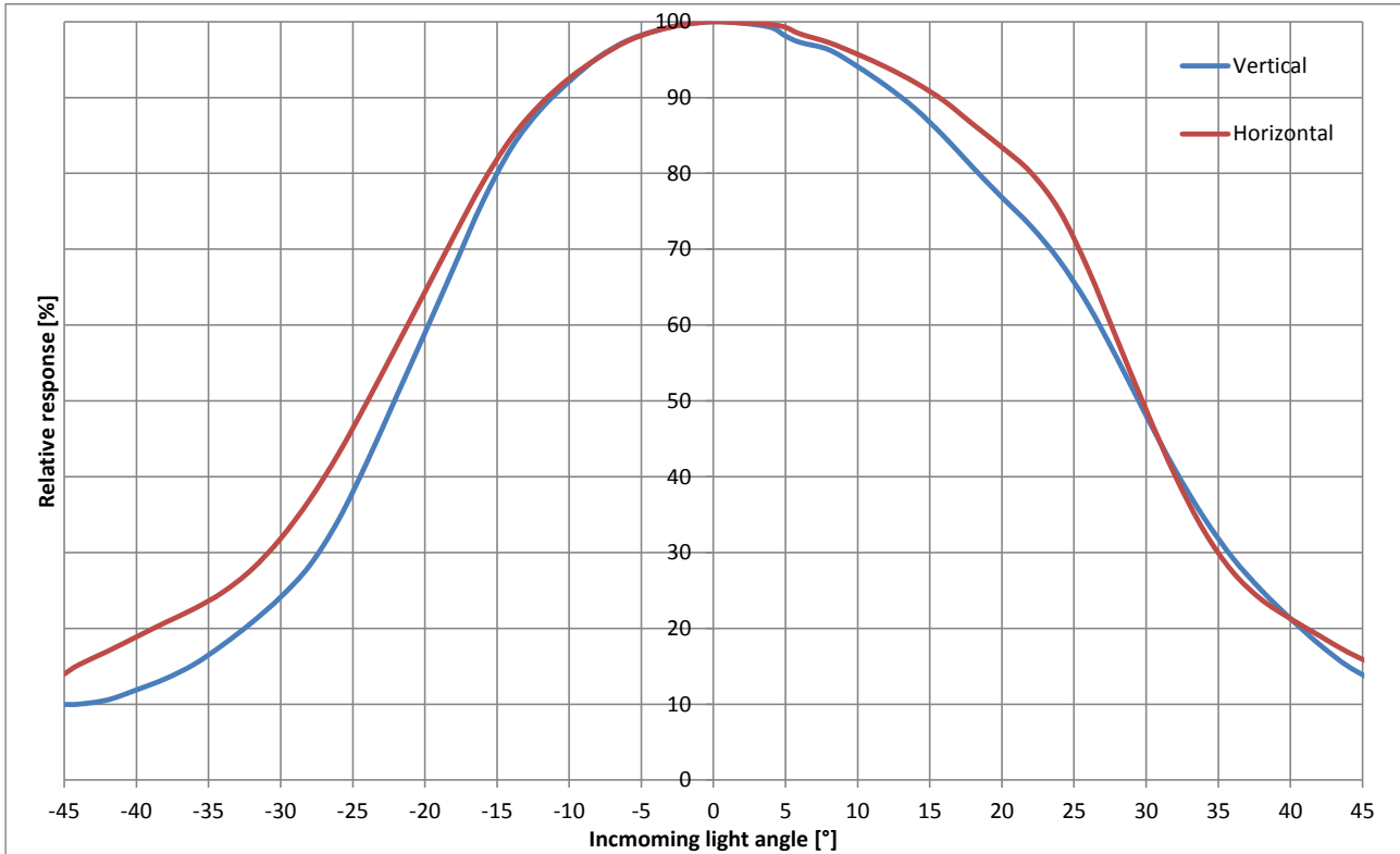
FIGURE 66: TYPICAL ANGULAR RESPONSE
