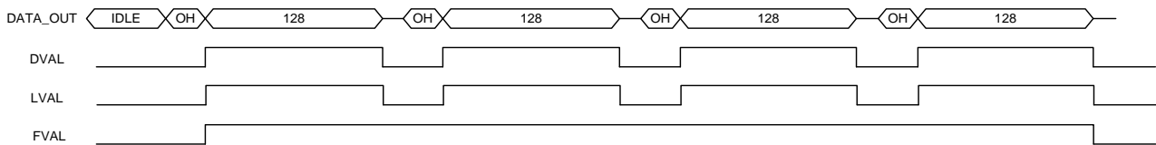
FIGURE 32: DVAL, LVAL AND FVAL TIMING IN 64CH OR 1X32CH OUTPUT MODE
