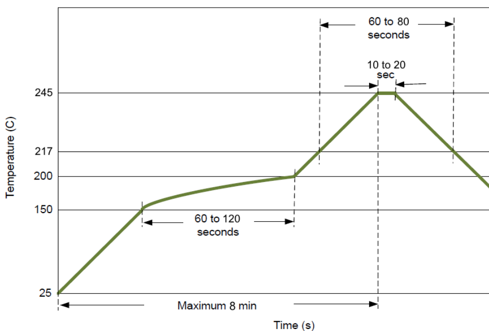
FIGURE 68: REFLOW SOLDERING
