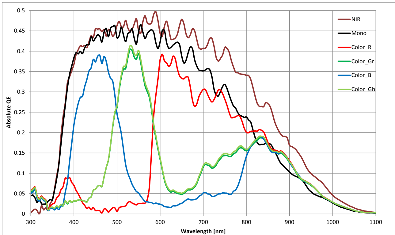
FIGURE 64: TYPICAL QE VS. WAVELENGTH
