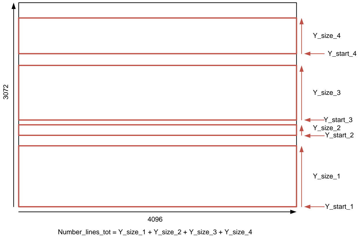
FIGURE 42: EXAMPLE OF 4 SUBWINDOWS READ-OUT
