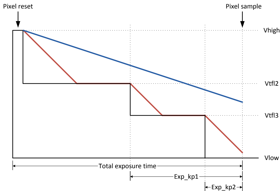
FIGURE 38: MULTIPLE SLOPE DETAILS
