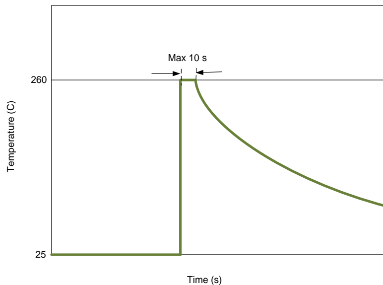
FIGURE 67: WAVE SOLDERING PROFILE
