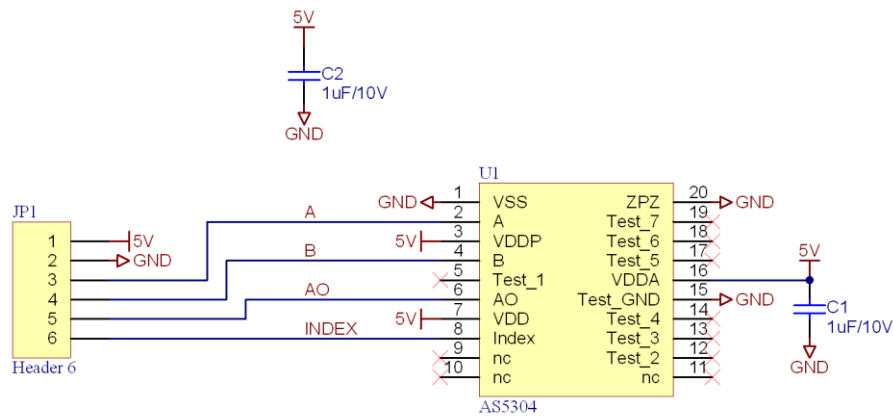
Figure 6: AS5304/AS5306-AB-2.1 schematics
