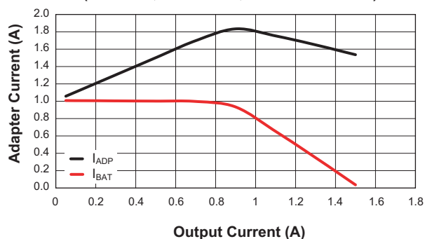
Adapter Charging Current vs. Output Current
