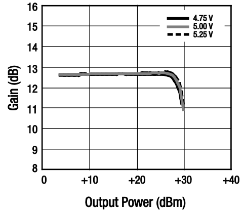
Figure 53. Gain vs Output Power Over Voltage
