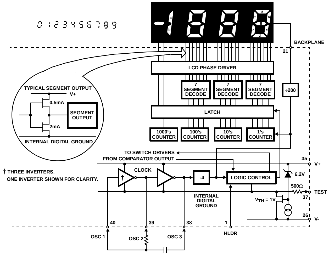
FIGURE 8. DIGITAL SECTION
