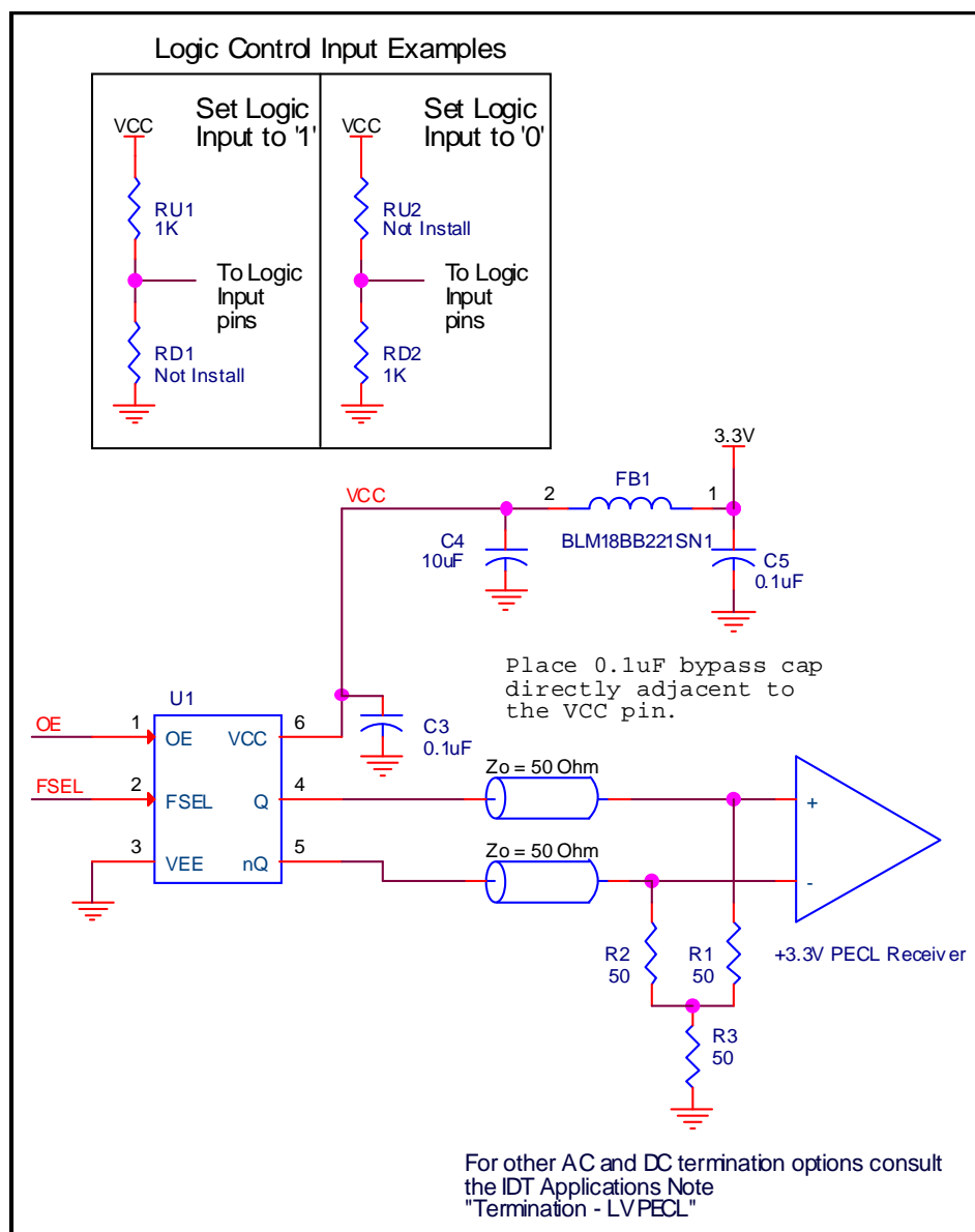
Figure 3. IDT8N3D085 Application Schematic
