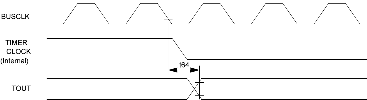
Figure 9. Timer Output Timing Diagram
