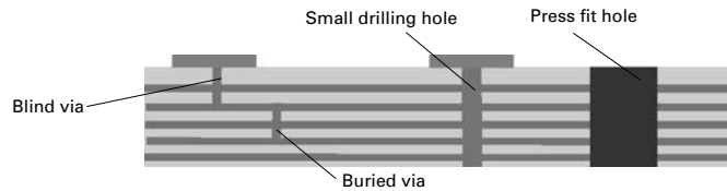
Cross-section showing PCB holes required for press-fit connections compared to small drilling holes or vias for CMT
