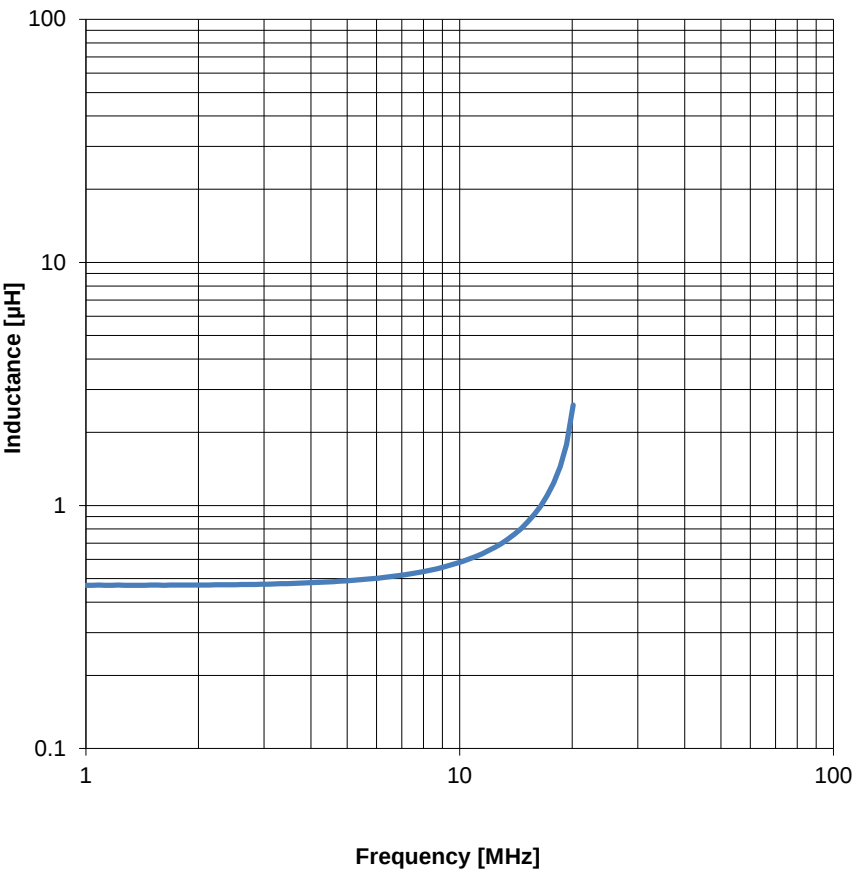
Typical Inductance vs. Frequency Characteristics:
