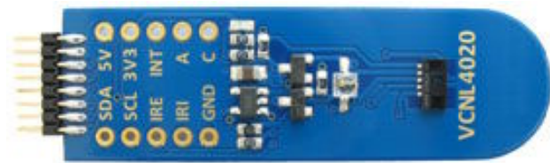
Fig. 5 - VCNL4020 Sensor Board
