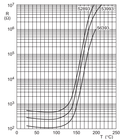
TYPICAL RESISTANCE/TEMPERATURE CHARACTERISTIC for 2322 660 52893/53993/56393.
