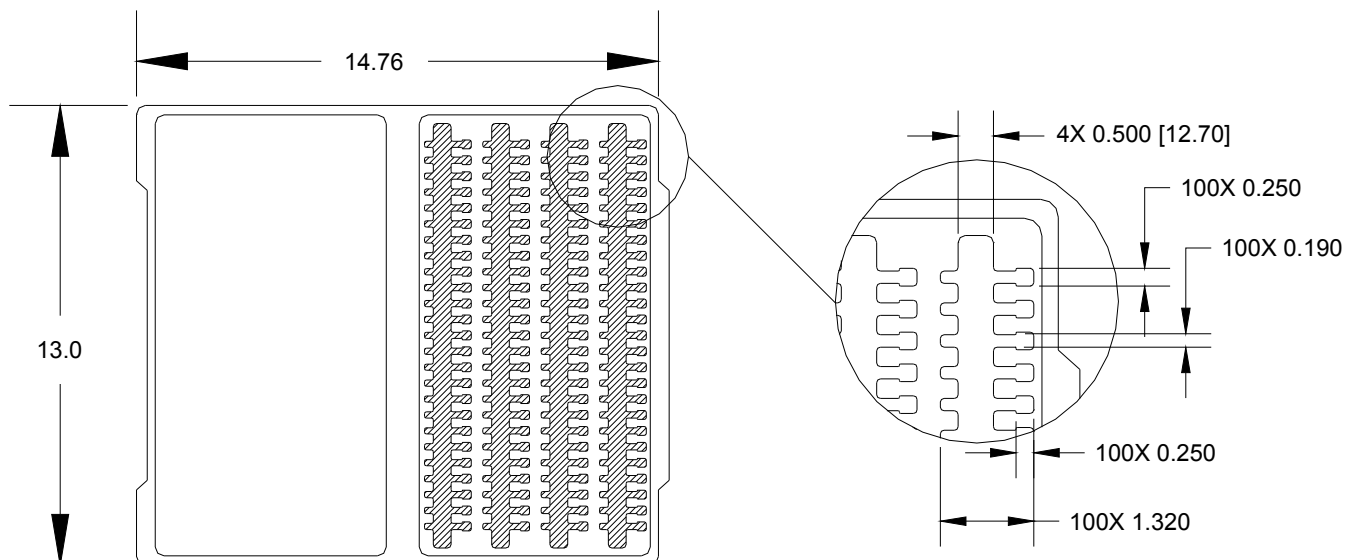
POCKET DETAIL
