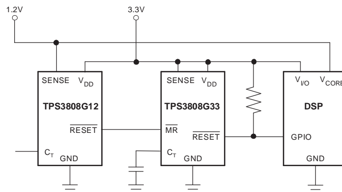
Figure 10. Using \overline{MR} to Monitor Multiple System Voltages
