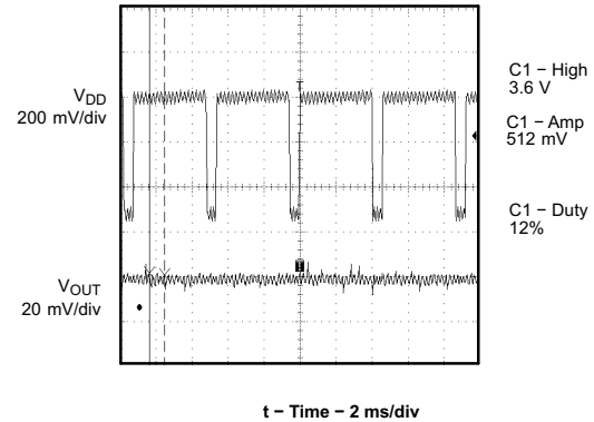
Figure 22. GSM Power Supply Rejection vs Time
