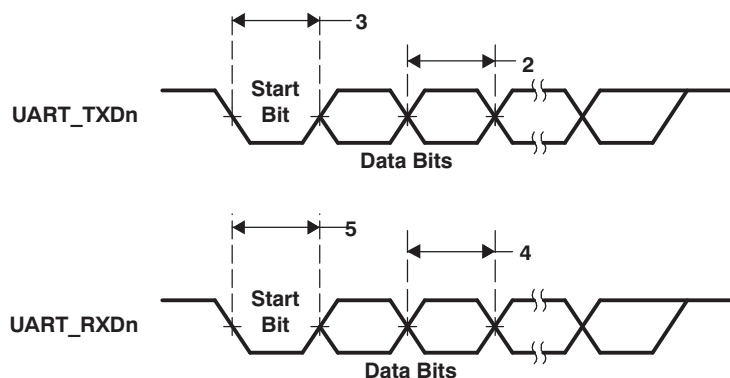
Figure 6-33. UART Transmit/Receive Timing
