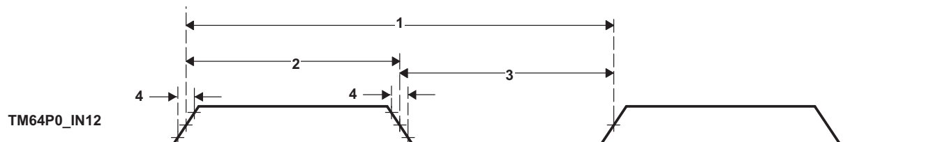
Figure 6-42. Timer Timing
