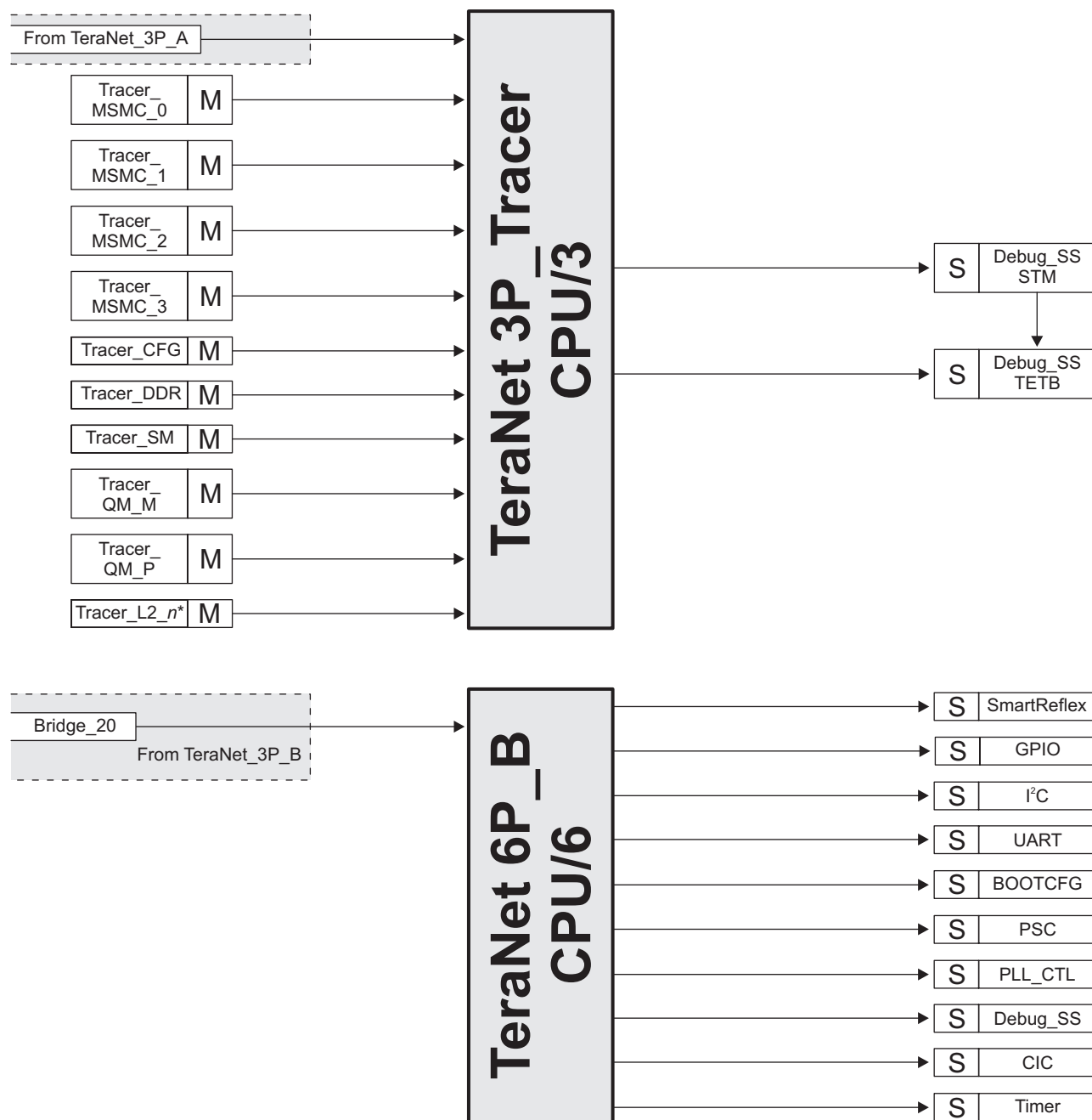
Figure 4-4 TeraNet 6P_B and 3P_Tracer for C6671
