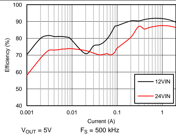
Figure 6. Efficiency at 85^\circ\text{C}
