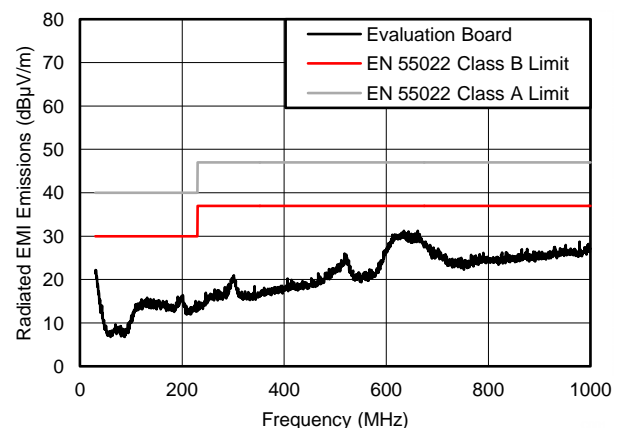
LM43602PWPEVM Radiated Emission Graph 12V_{IN} to 3.3V_{OUT} F_s = 500 kHz I_{OUT} = 2 A
