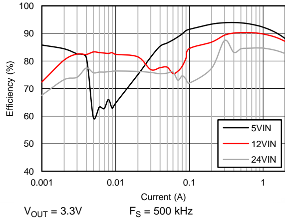
Figure 3. Efficiency at 85^\circ\text{C}
