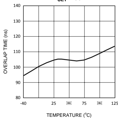
Overlap Time vs Temperature R SET = 38K
