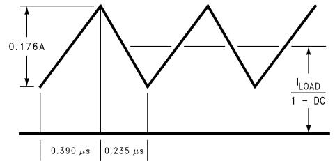
Figure 27. 10 µH Inductor Current, 5V–12V Boost (LM2733X)
