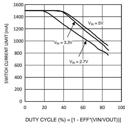
Figure 28. Switch Current Limit vs Duty Cycle - "X"
