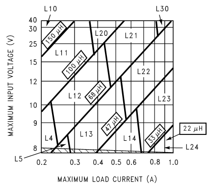
Figure 10. LM2675-5.0
