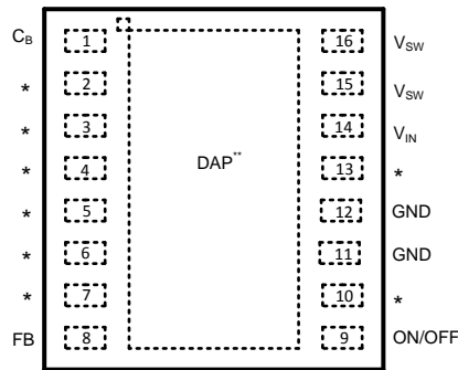
Figure 1. LLP Package
