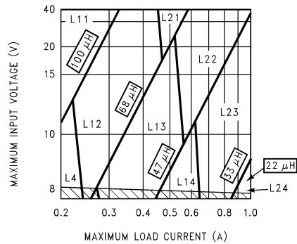
Figure 9. LM2675-3.3
