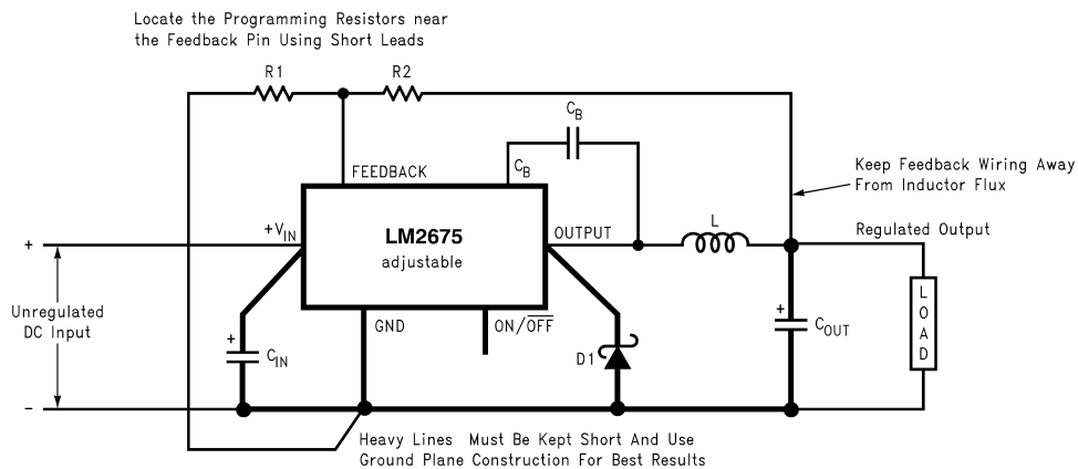
Figure 7. Standard Test Circuits and Layout Guides Fixed Output Voltage Versions
