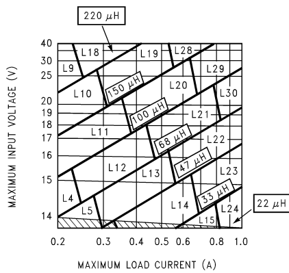
Figure 11. LM2675-12
