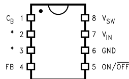
Figure 2. SO-8/DIP Package
