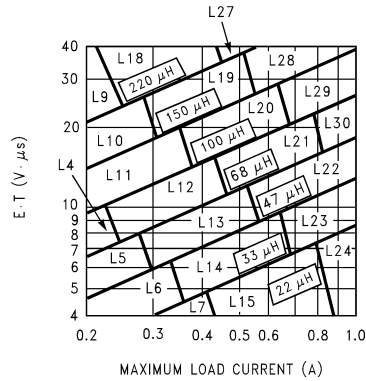
Figure 12. LM2675-ADJ
