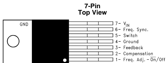
Figure 1. LM2588T-12 or LM2588T-ADJ See Package Number NDZ0007B
