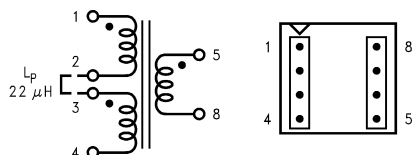
Figure 39. T1 - Top View Renco RL-5530
